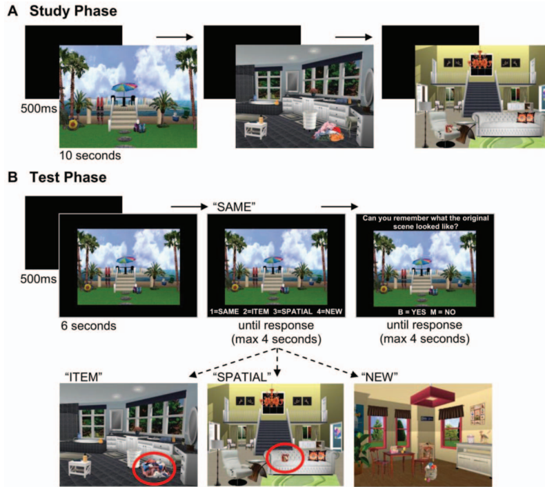
Figure 1. During the study phase (A), participants were shown a series of scenes, each for 10 s, separated by a blank screen for 500 ms. For each trial in the test phase (B), participants were presented with the scene for 6 s, after which the response options appeared and they had an additional 4 s in which to make their response. The scene could either be the SAME as the studied scene (trial shown), or could contain an ITEM or SPATIAL change (changes are circled in the figure for illustration purposes), or the scene could be NEW. After identification of the scene as the SAME or changed (ITEM or SPATIAL), participants were asked to indicate whether their response was based on recollection or not. See the online article for the color version of this figure.
